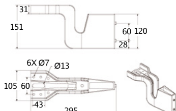
Platine Z standard
