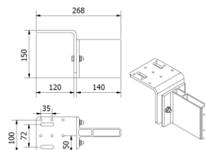
Platine Z standard
